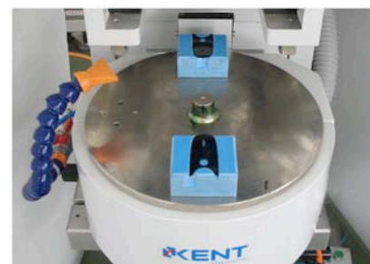
2-station motor drive turntable
